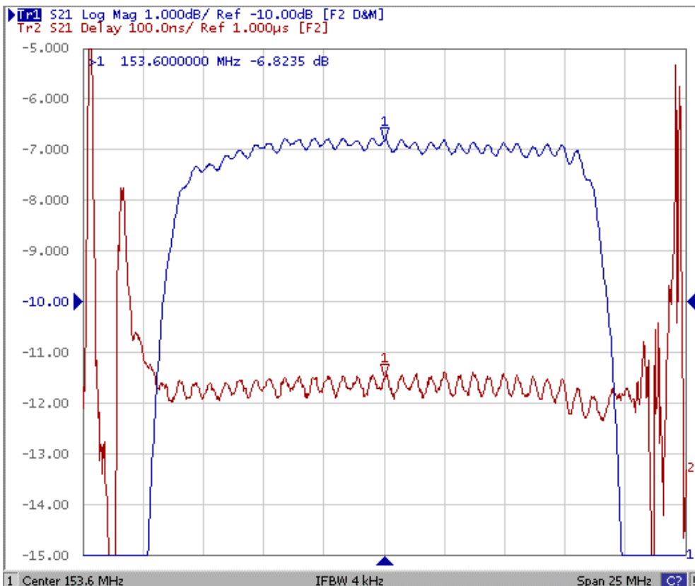
Fig2. Horizontal: 2.5MHz/Div Vertical: 100nec/Div
